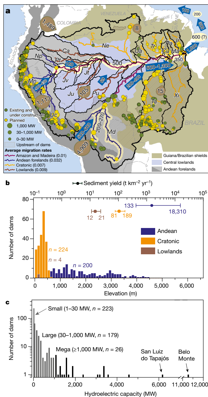
Figure 1 | The Amazon's 19 sub-basins: geologic–physiographic domains, sediment fluxes, channel migration rates and dams. a , The Andean foreland rivers are: Marañón (Mn), Ucayali (Uc), Napo (Np), Putumayo (Pt) and Caqueta-Japura (Ca). The cratonic rivers are: Jari (Jr), Paru (Pa), Curuapenema (Cu), Maricuru (Ma), Tapajós (Ta), Xingu (Xi), Trombetas (Tr), Negro (Ne) and Uatumbá (Ua). The mixed-terrain river is: Madeira (Md). The lowland rivers are: Juruá (Ju), Purús (Pu), Jutai (Jt) and Javari (Jv). Averaged sediment yield ( \text{t km}^{-2} \text{yr}^{-1} ) for major sediment source terrains is shown as brown 'balloons' 12,20 ; sediment loads ( \text{Mt yr}^{-1} ) are shown as yellow shading 12,18 ; and mean channel migration rates (channel widths per year) are shown by physiographic province 23 (red, green and blue lines). Migration rates of 0.01 were estimated for the Solimões–Amazon and Madeira rivers (purple line). b , Numbers of dams in each elevation range (bars) and geological region (Andean mountains, cratonic and lowlands). Ranges and means of sediment yields ( \text{t km}^{-2} \text{yr}^{-1} ) measured in each region are shown along the upper x axis. c , Histogram of the number of dams scaled by their hydroelectric capacity.
